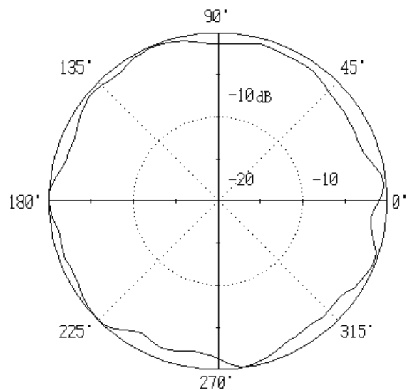
H Plane
