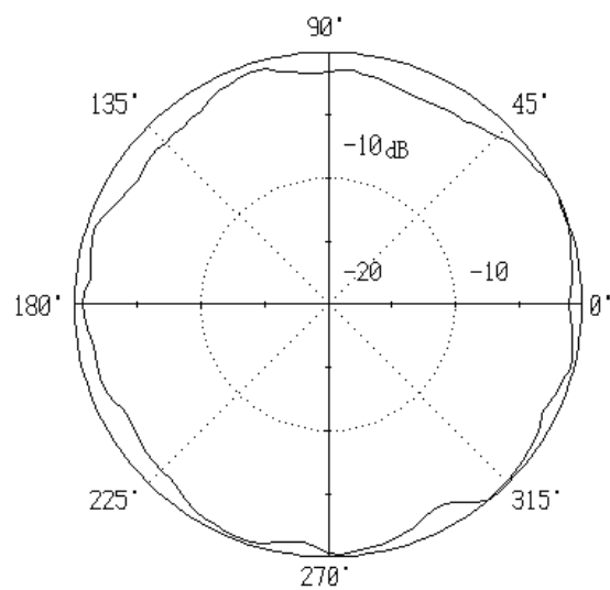
H Plane
