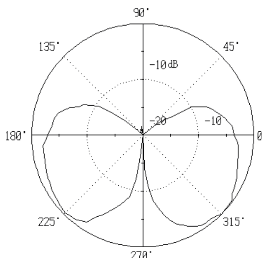
E Plane
