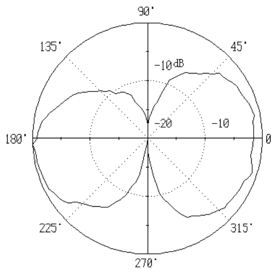
E Plane
